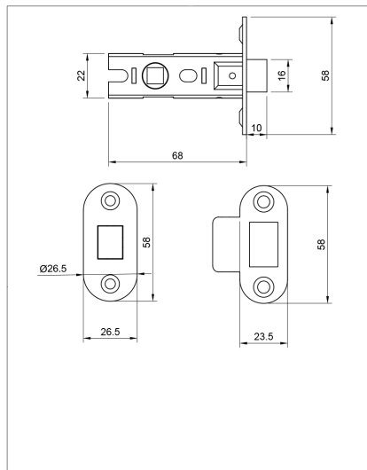
Product Finish Pictured: Antique Brass (AB)
