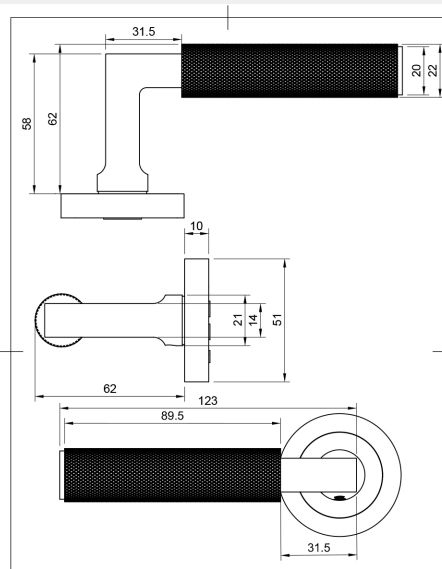
Finish Photographed: Satin Nickel
